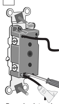
Press in slot and pull out wire
