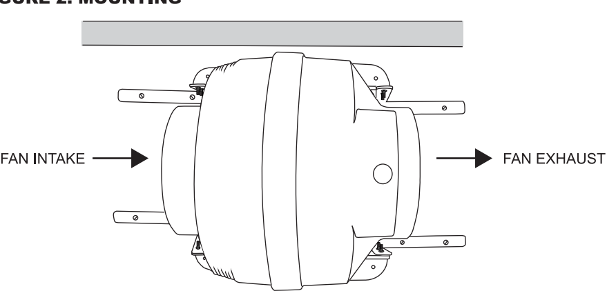
FIGURE 2: MOUNTING
