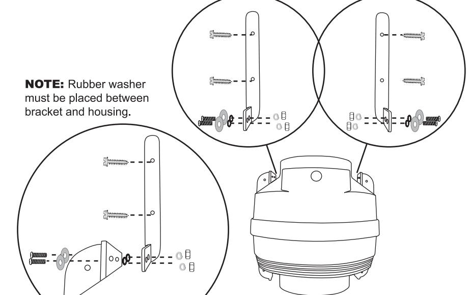
FIGURE 1: MOUNTING BRACKETS
