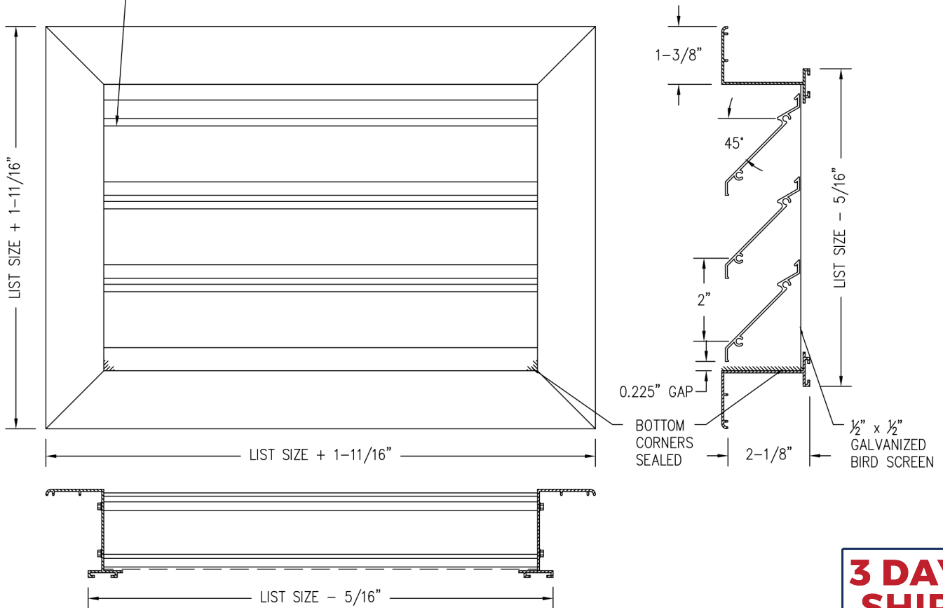
STORMPROOF BLADES ON 45° DEFLECTION AND 2" SPACING
