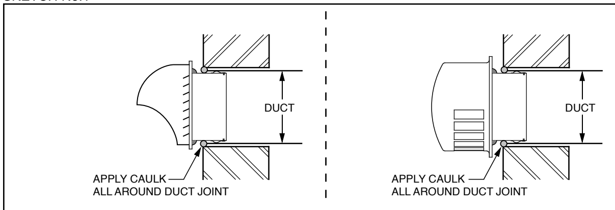
SKETCH No.2
